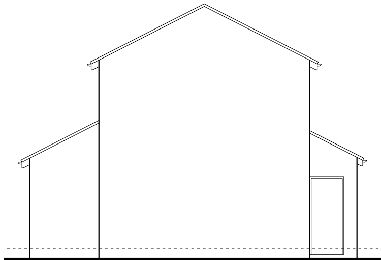
SIDE ELEVATION 1:100
