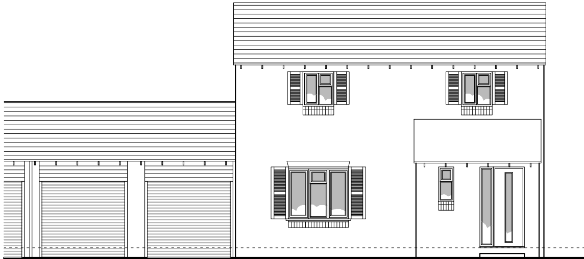
FRONT ELEVATION 1:100
