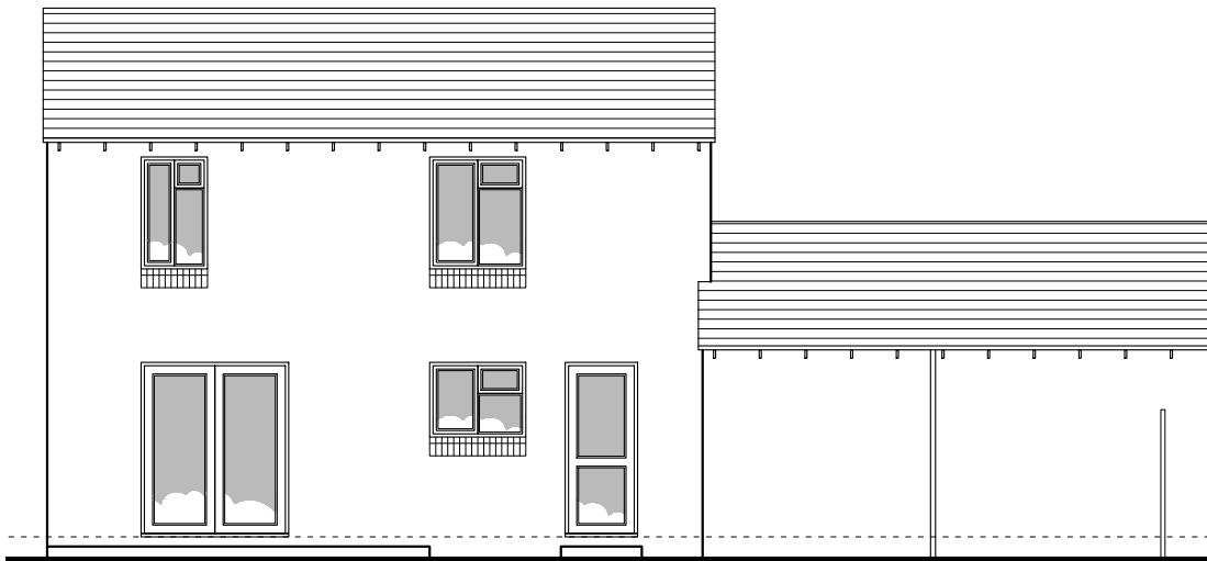
REAR ELEVATION 1:100
