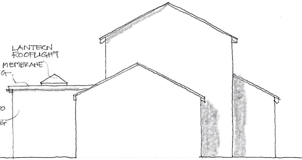
SIDE ELEVATION 1:100
