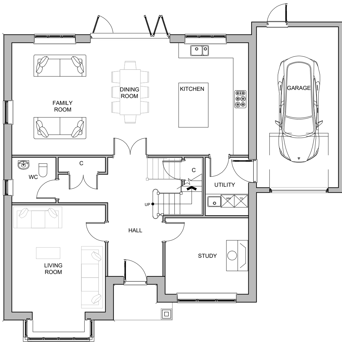
PLOT 4 & 5 GROUND FLOOR PLAN
