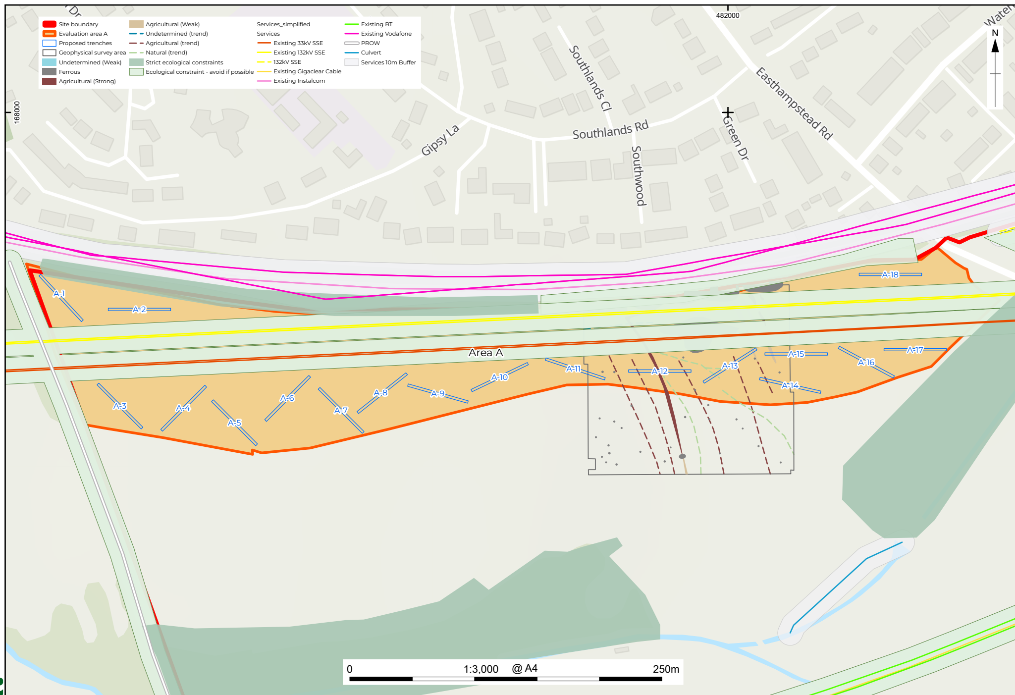
Figure 4: Proposed trench location
