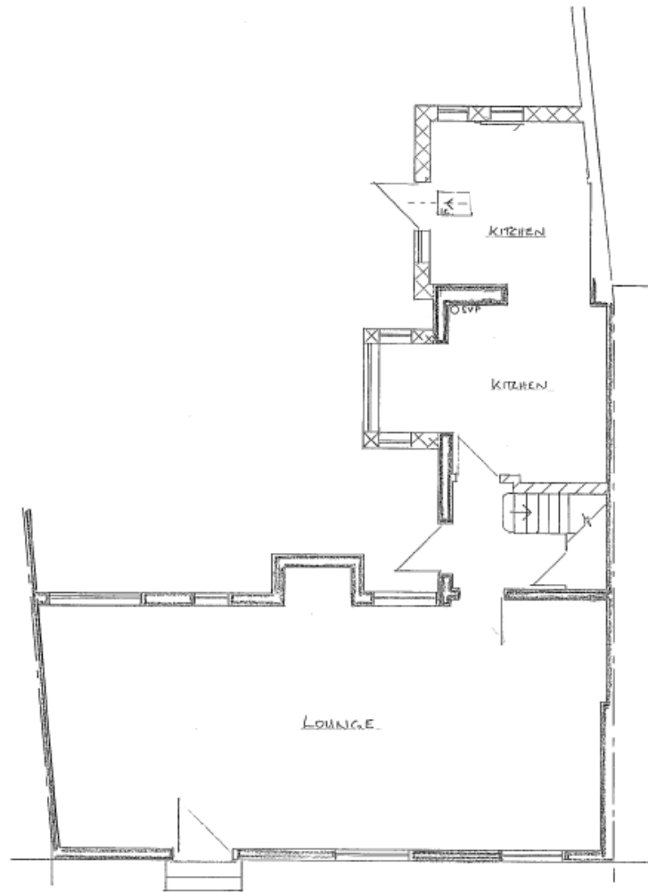
Ground Floor Kitchen Plan as Existing
