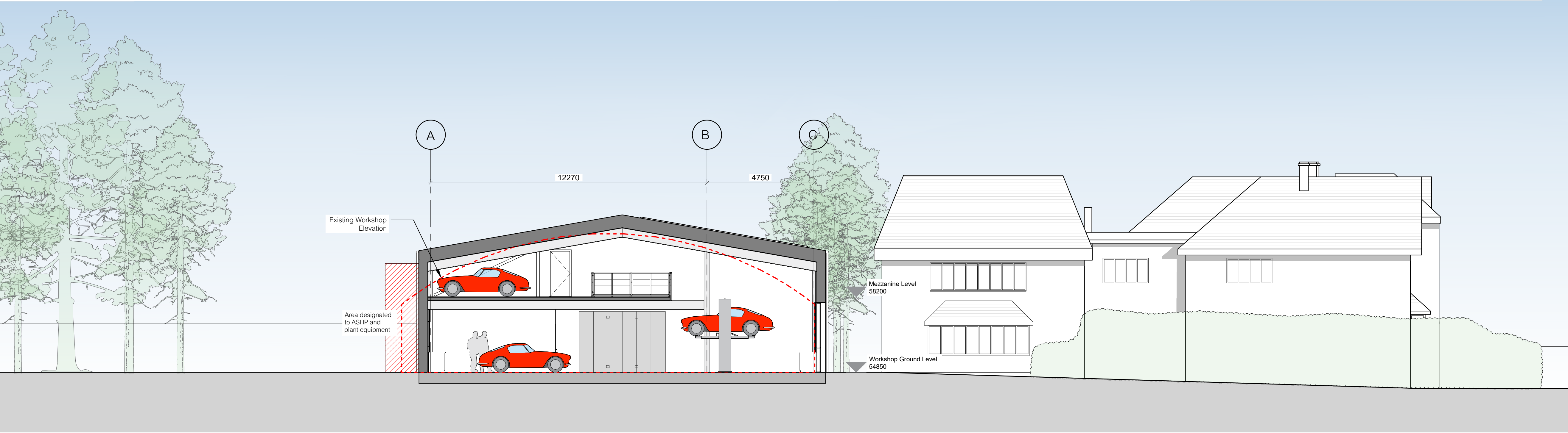
2 Proposed Short Section 1:100
