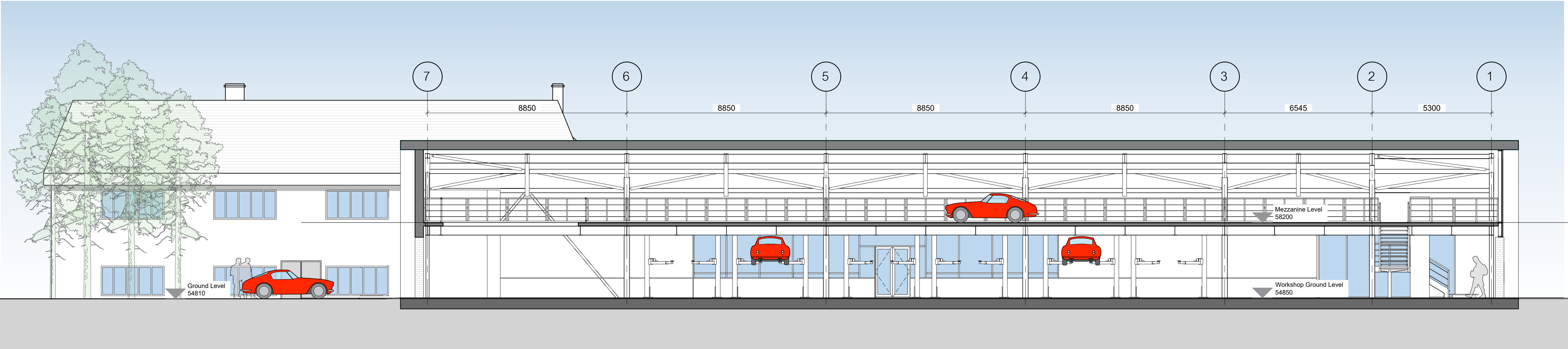
1 Proposed Long Section 1:100
