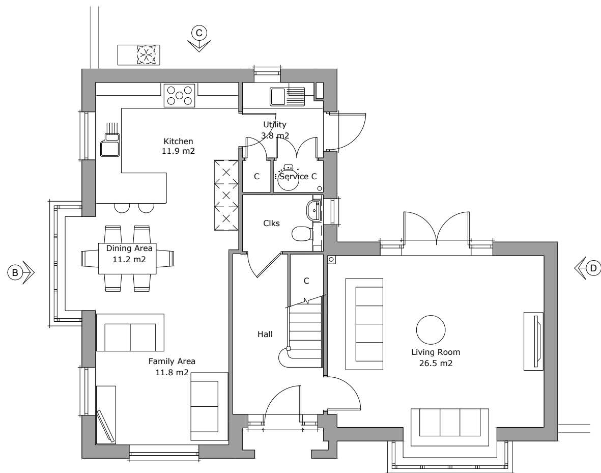
Ground Floor Plan Area 83.5m²
