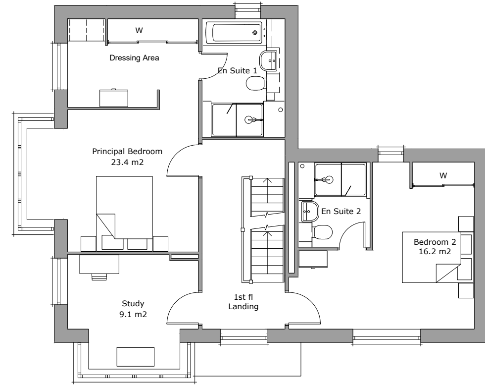
First Floor Plan Area 75.9m 2
