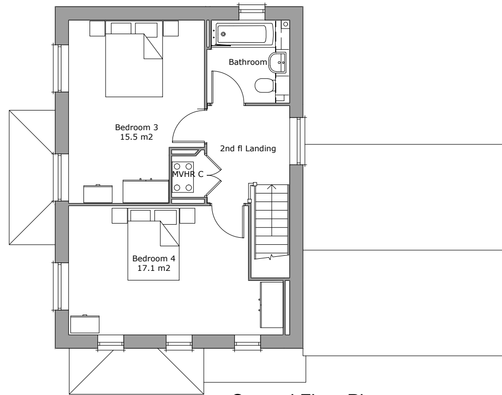
Second Floor Plan Area 48.2m 2
