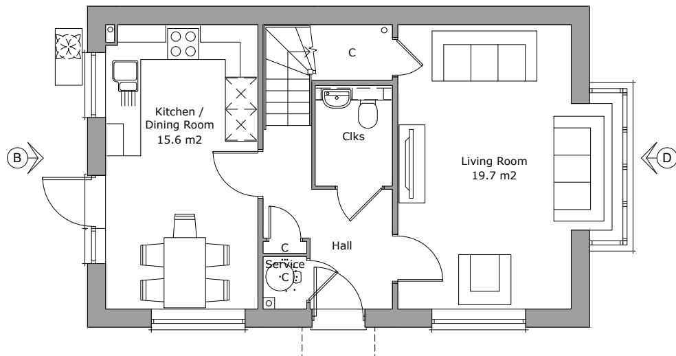
Ground Floor Plan Area 51.0m 2
