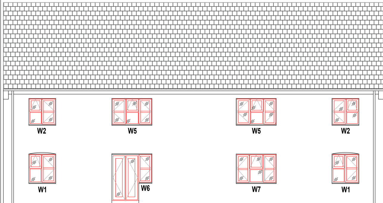
1-7 GELDER CLOSE PROPOSED REAR ELEVATION VIEW C 1:100
