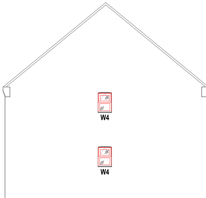
1-7 GELDER CLOSE PROPOSED SIDE ELEVATION VIEW D 1:100
