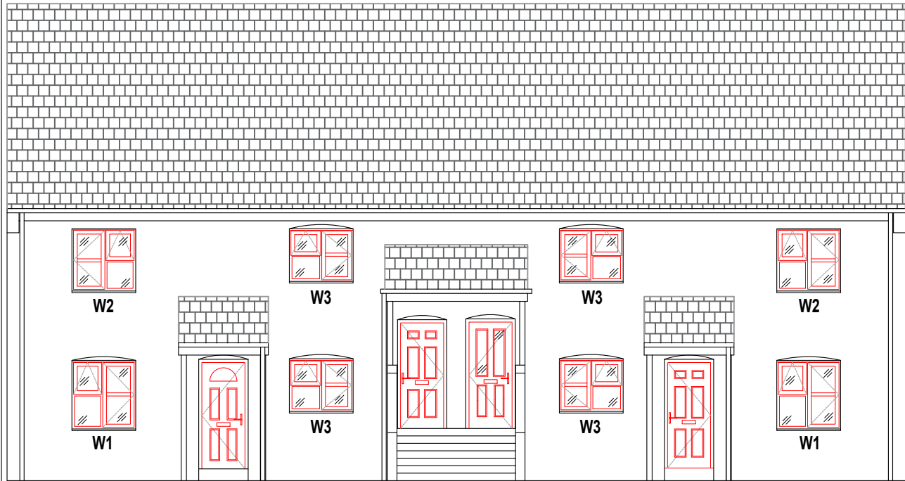
1-7 GELDER CLOSE PROPOSED FRONT ELEVATION VIEW A 1:100
