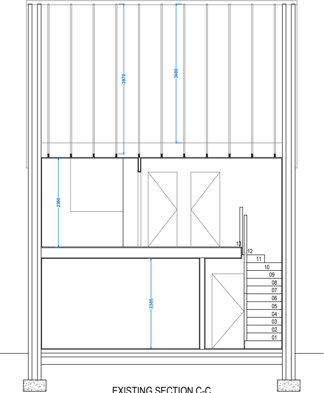
EXISTING SECTION C-C
