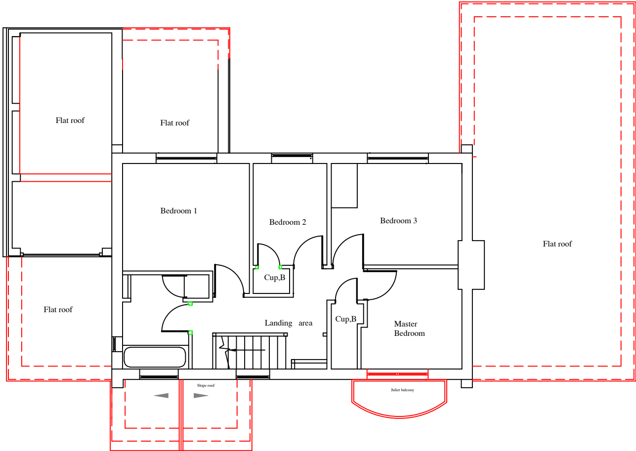
PROPOSED FIRST FLOOR
