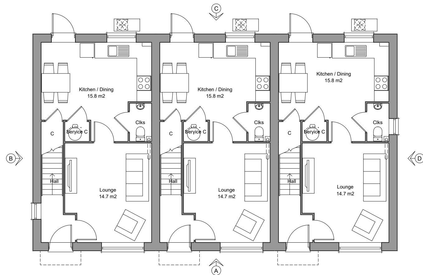
Ground Floor Plan Area 40.0m²
