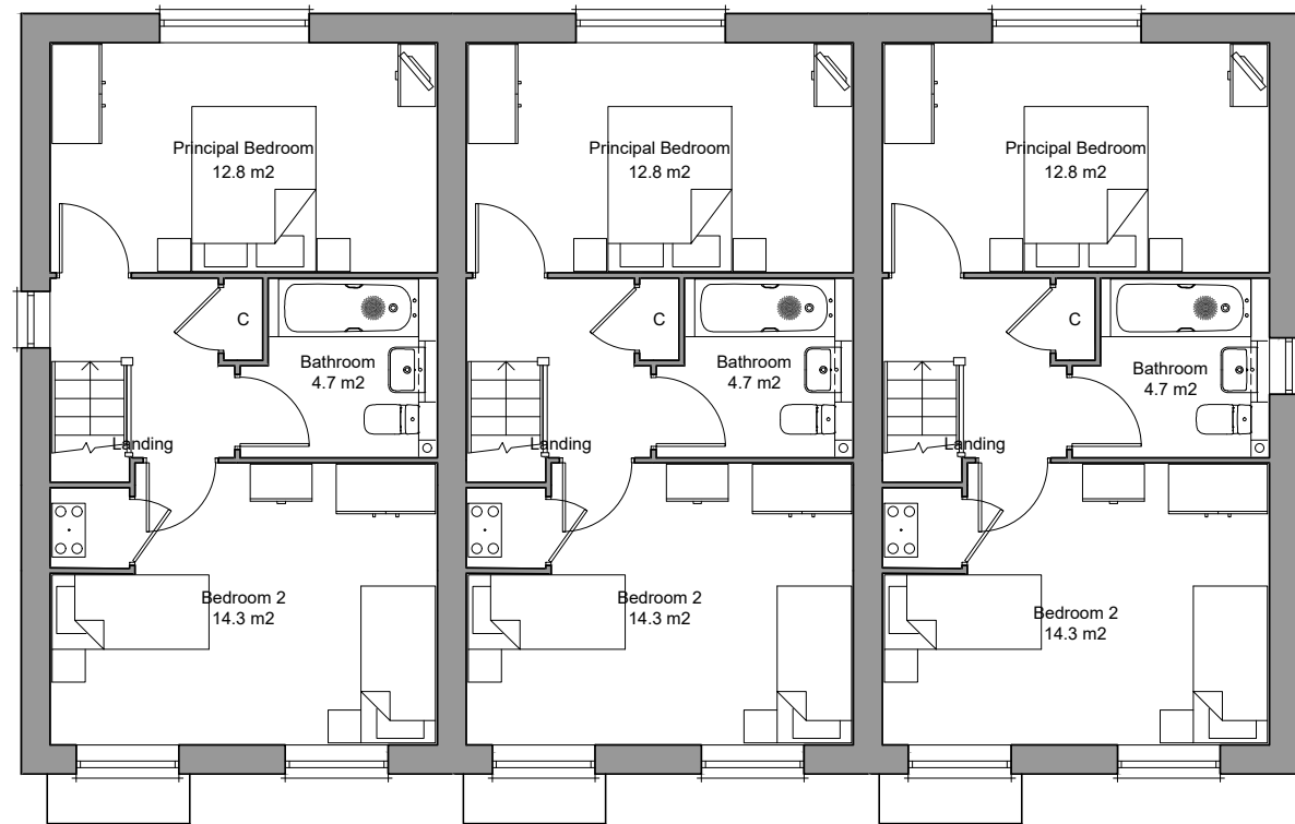
First Floor Plan Area 40.0m²
