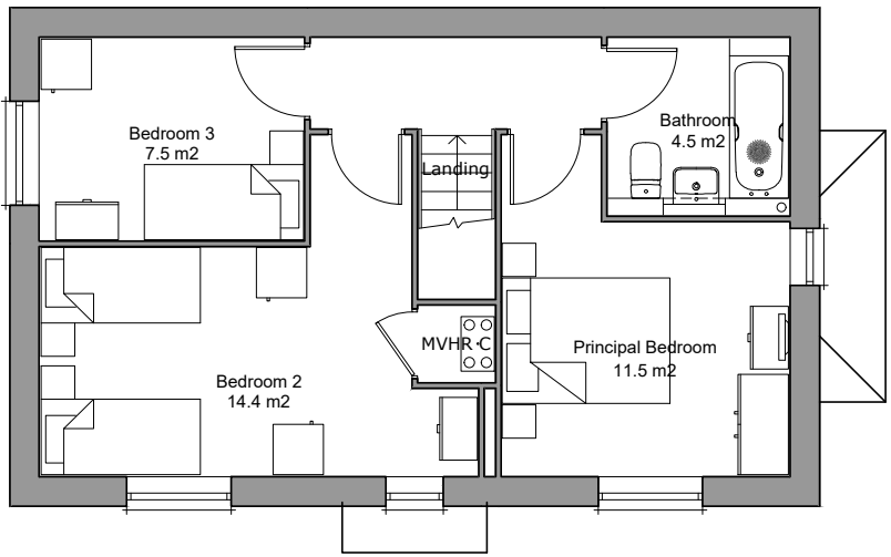
First Floor Plan Area 47.1m²
