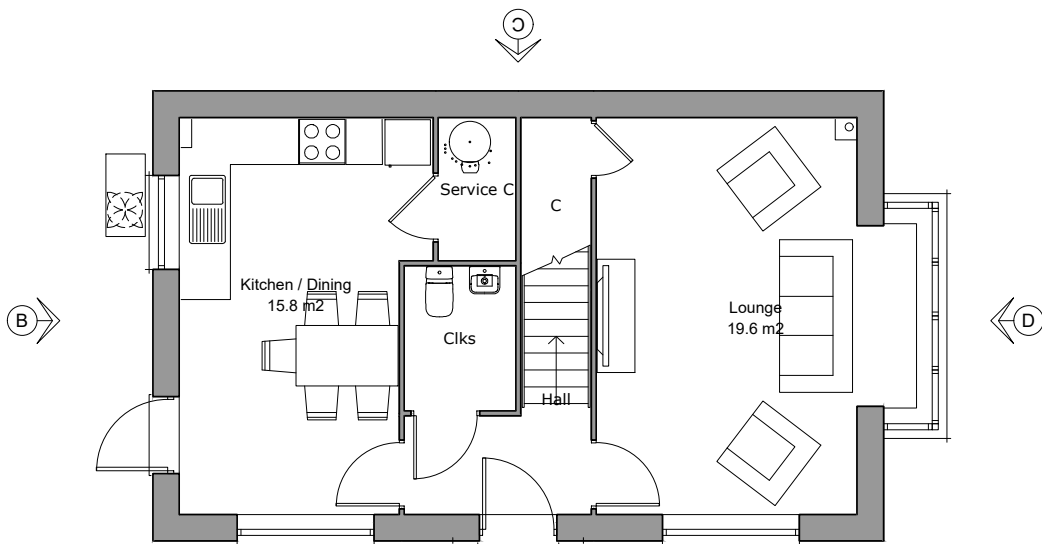
Ground Floor Plan Area 49.0m²
