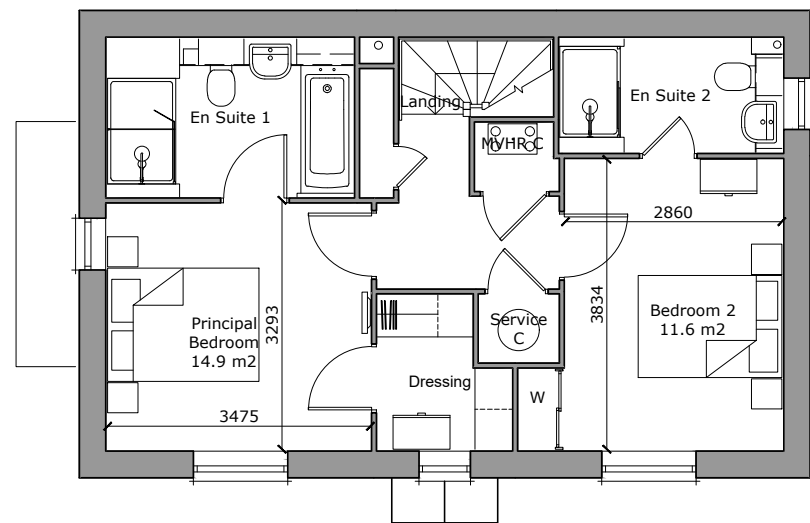
First Floor Plan Area 49.1m²
