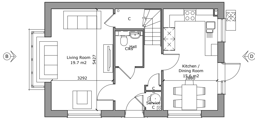
Ground Floor Plan Area 51.0m²
