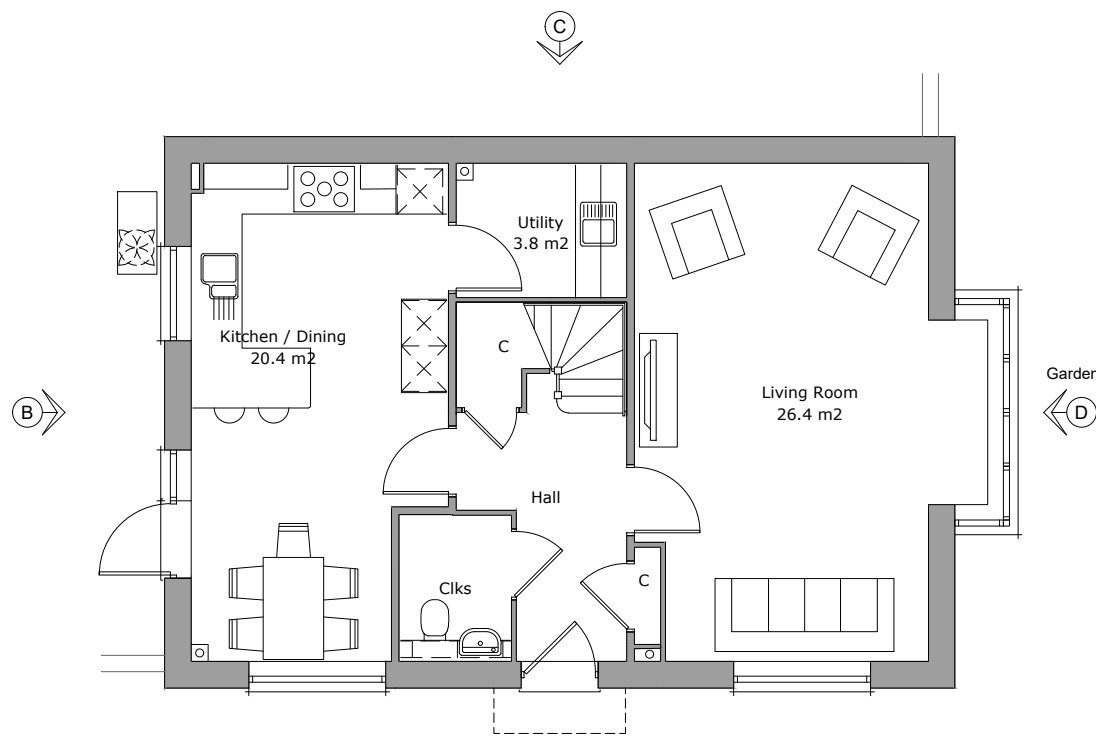
Ground Floor Plan Area 66.2m²
