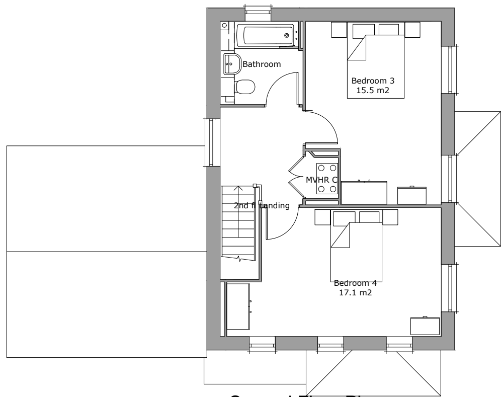
Second Floor Plan Area 48.2m²
