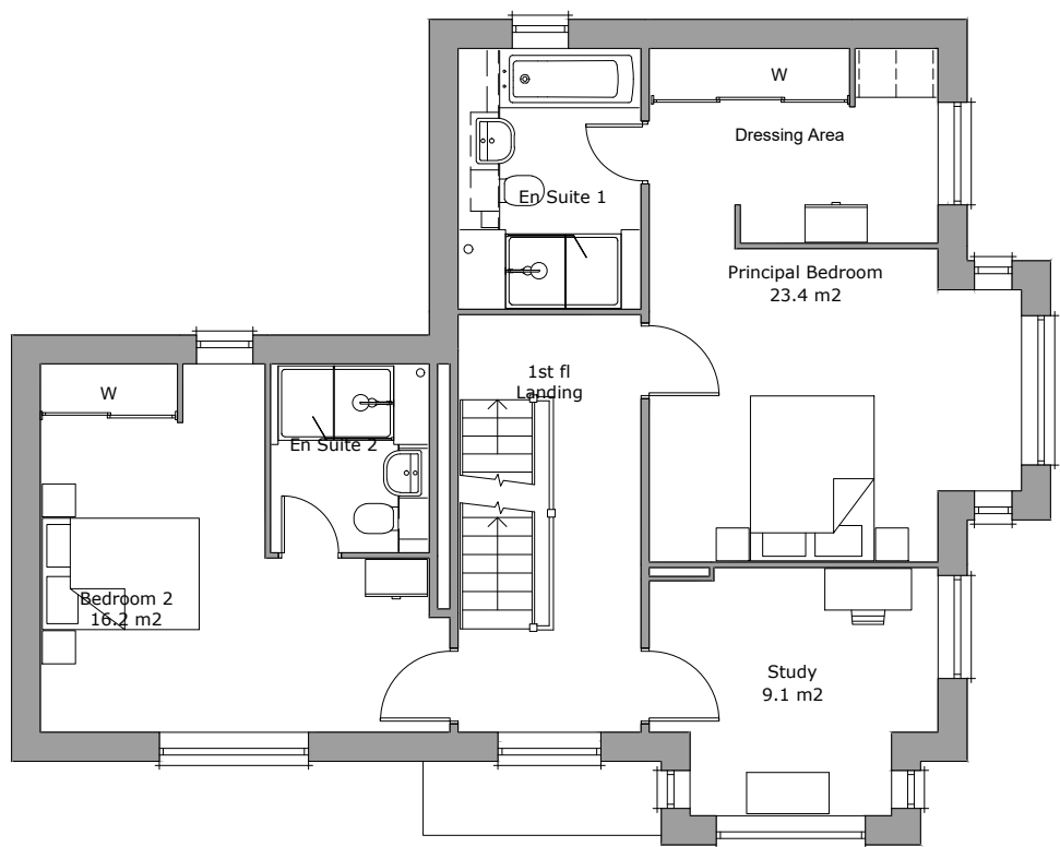
First Floor Plan Area 75.7m²
