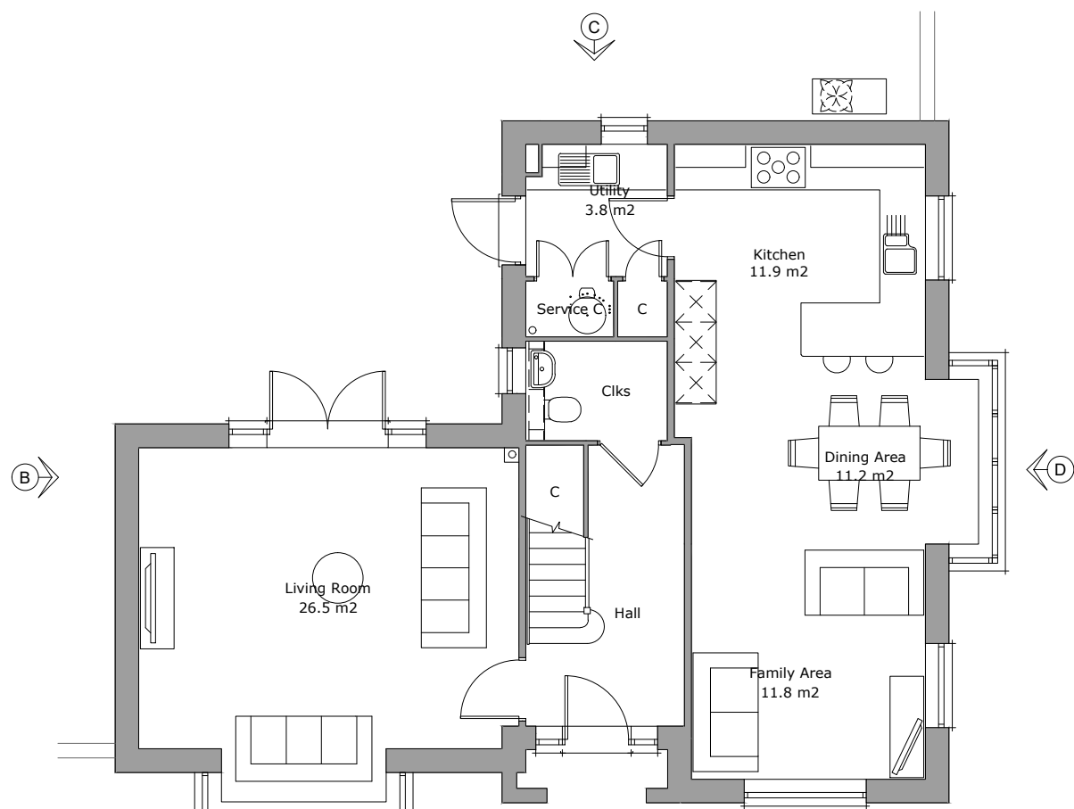
Ground Floor Plan Area 83.5m²
