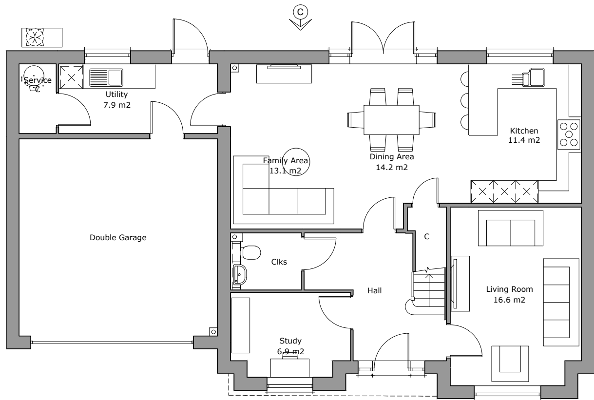
Ground Floor Plan Area 91.0m 2
