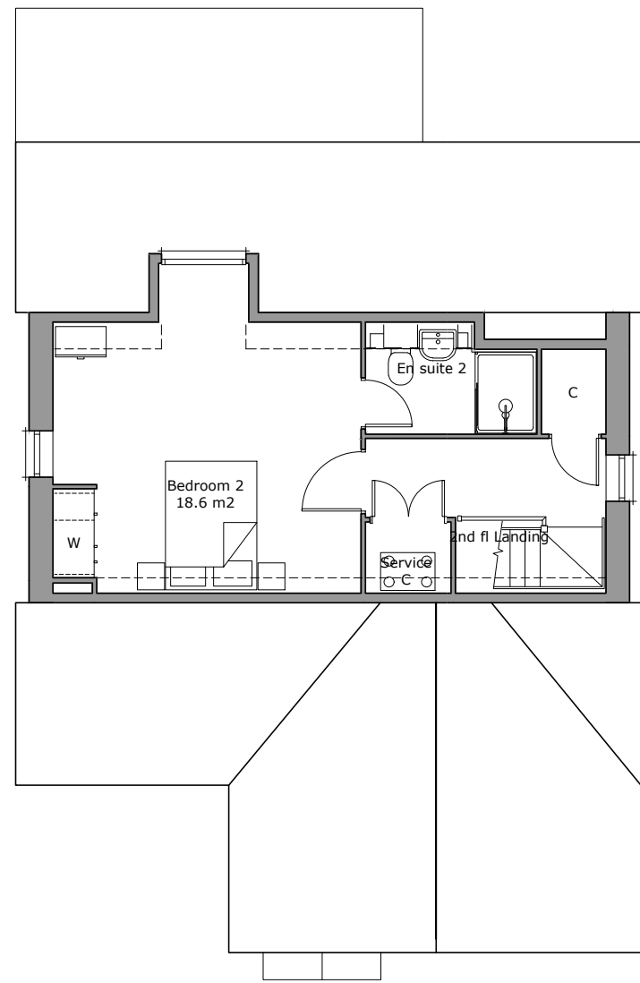
Second Floor Plan Area 33.2m²
