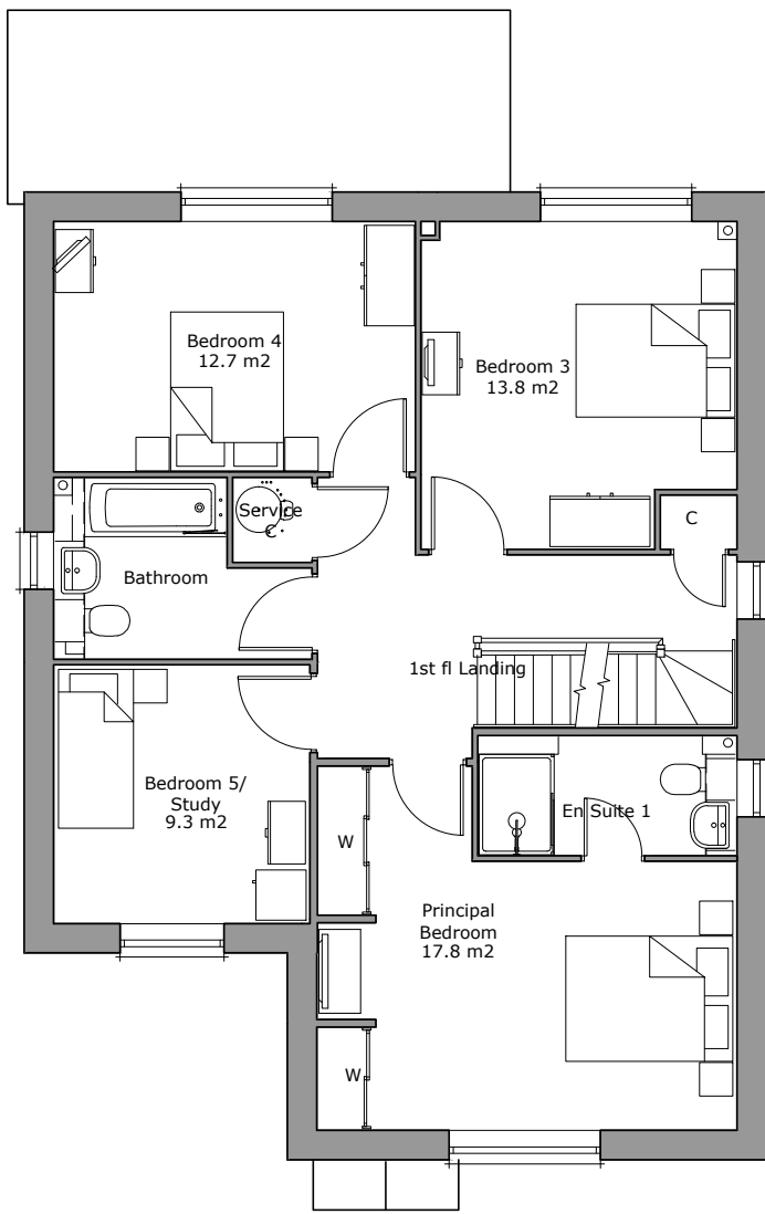
First Floor Plan Area 81.1m²
