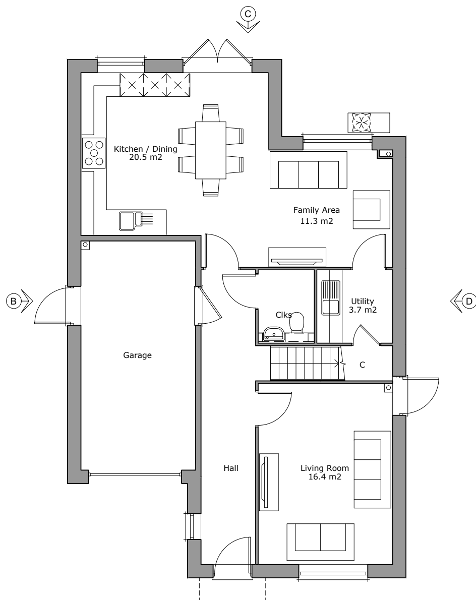
Ground Floor Plan Area 71.7m²
