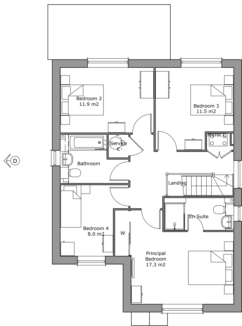
First Floor Plan Area 74.7m²
