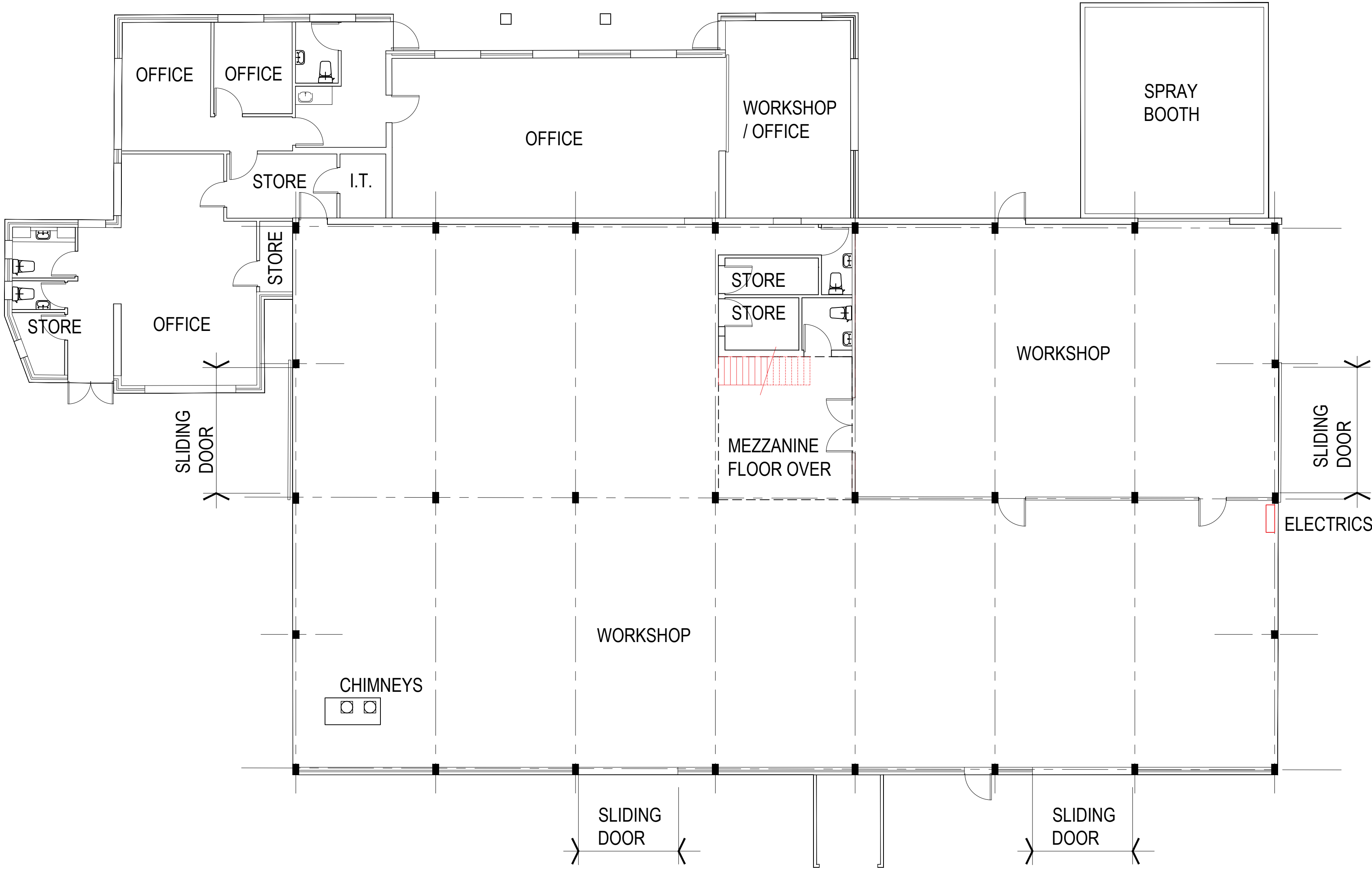
EXISTING WORKSHOP - GROUND FLOOR LAYOUT (SCALE 1:100)
