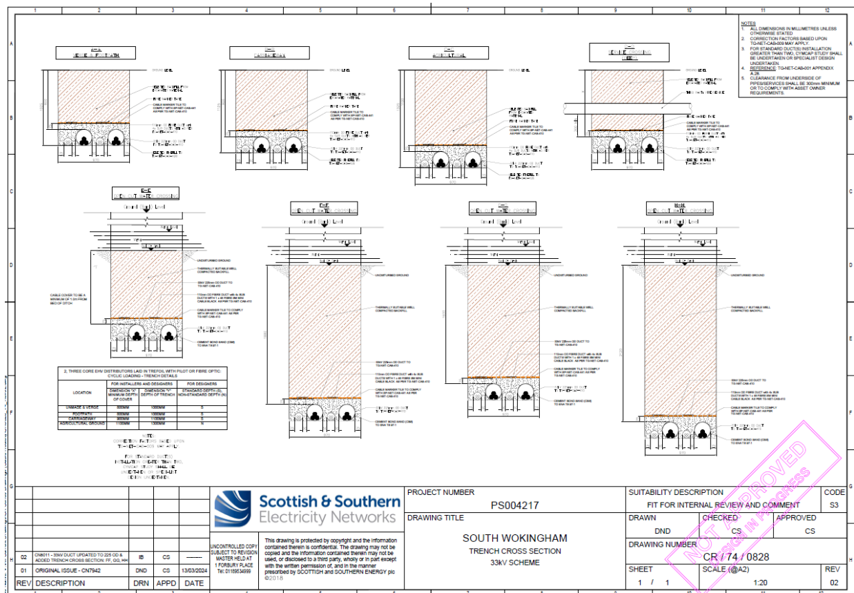
Figure 15: Phase 0 - 33 kV Single trench design
