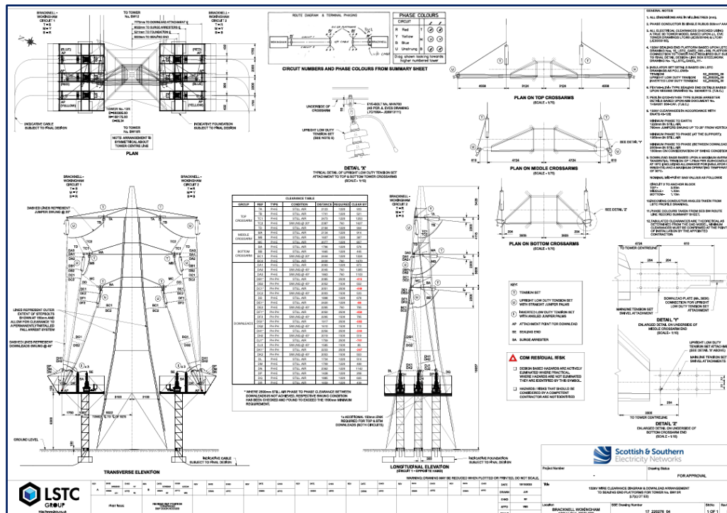
Figure 12: Indicative 132kV Terminal Tower designs
