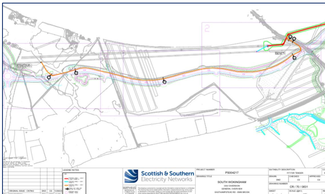
Figure 8: Phase 2 33kV Diversion Route
