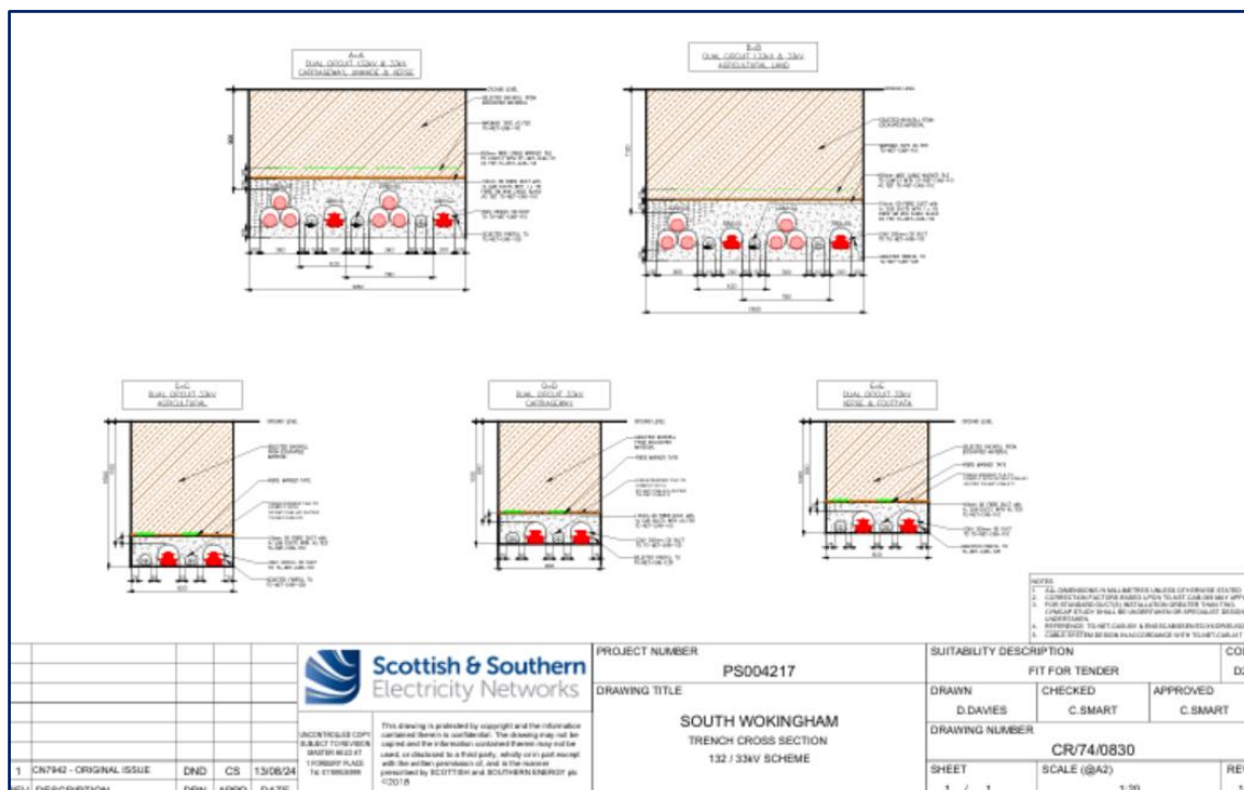
Figure 13: Phase 1 - 33kV and 132kV shared trench
