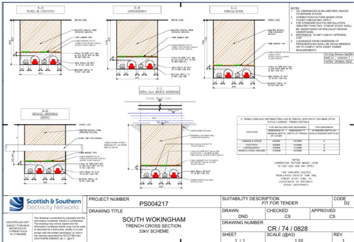
Figure 14: Phase 2 - 33kV single trench
