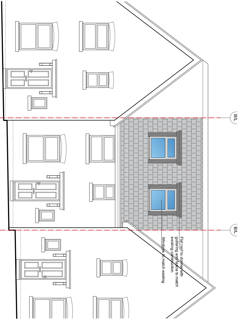
FRONT ELEVATION AS PROPOSED 26 WHITETHRON, SHINFIELD - RG2 9GF
