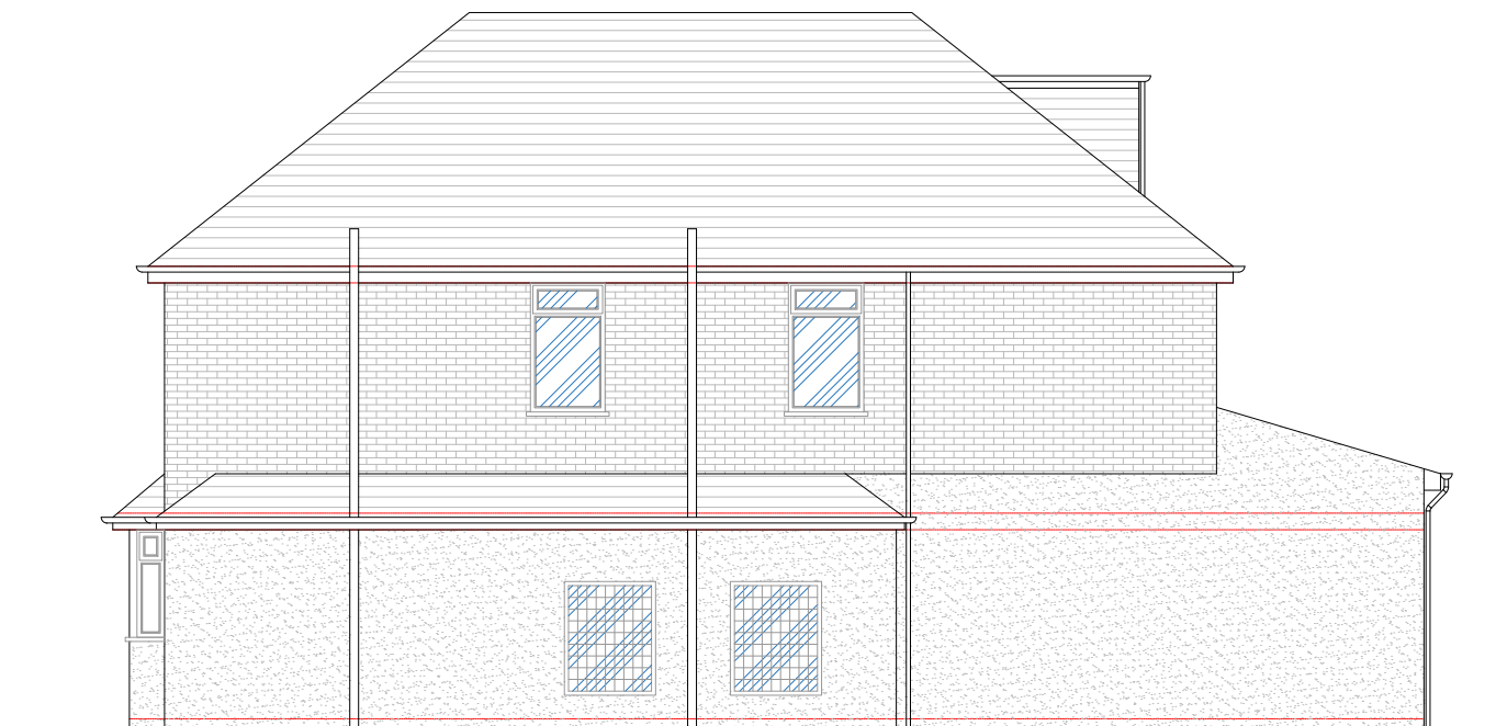
Existing Right Elevation
