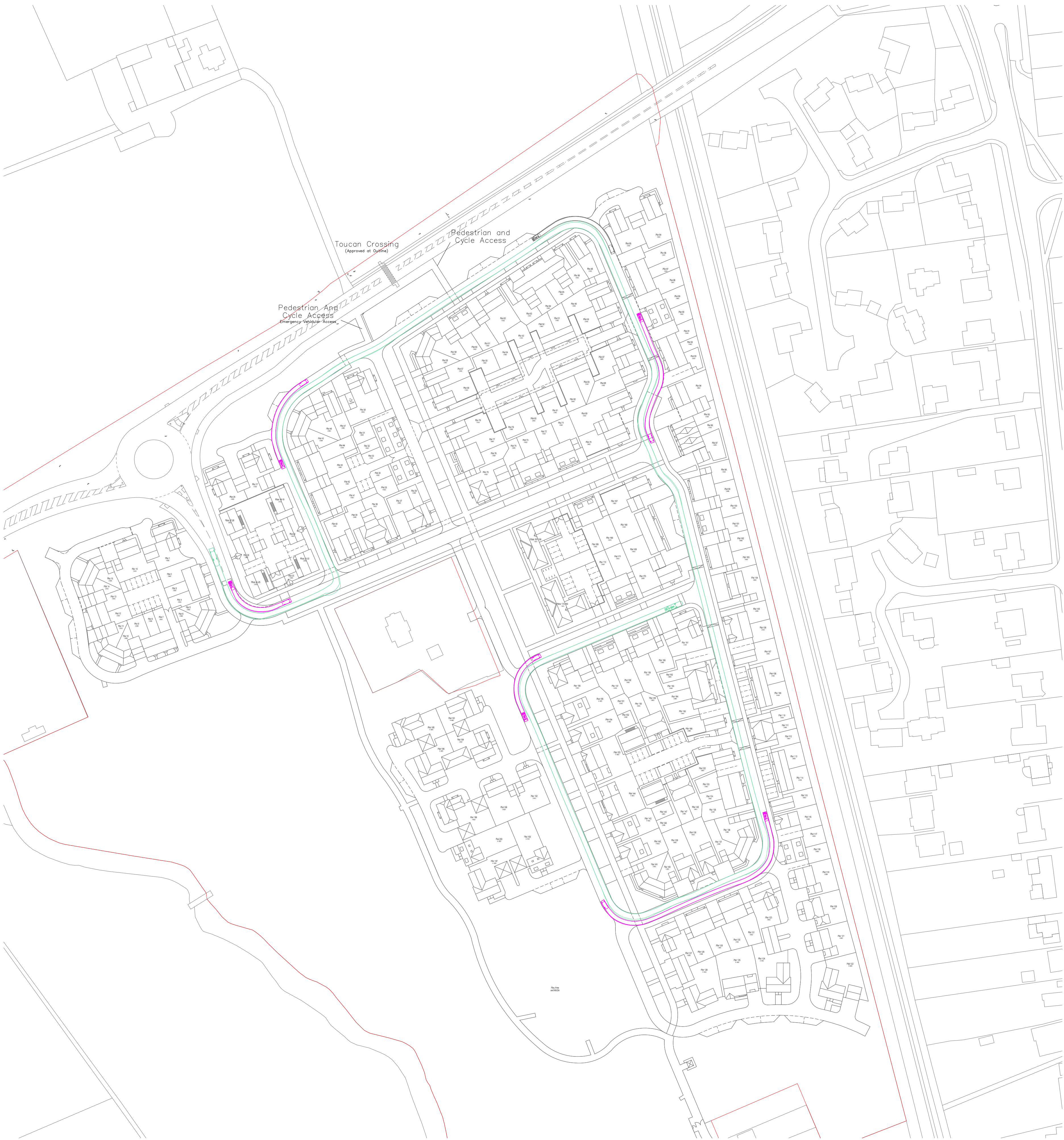
Fire Vehicle Tracking (With Car Passing) Scale - 1:1000
