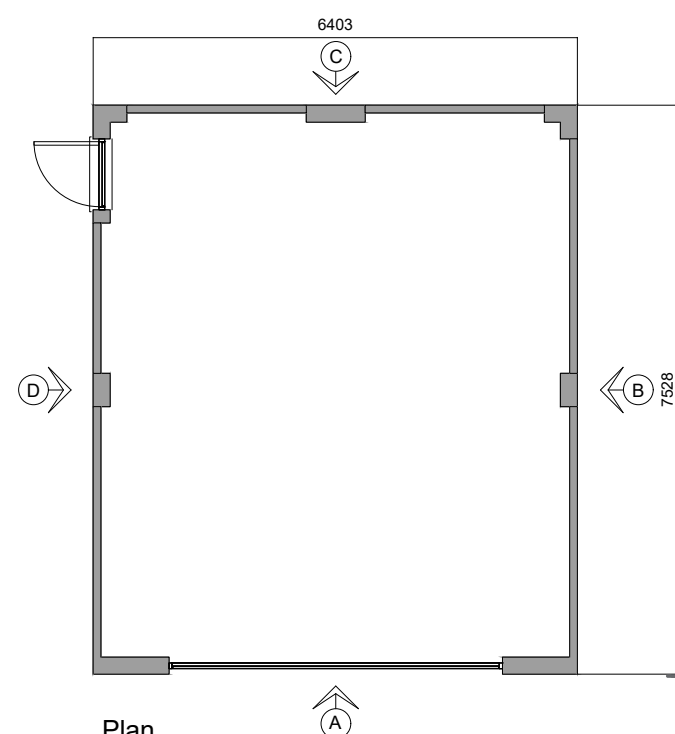
Plan Plot 30
