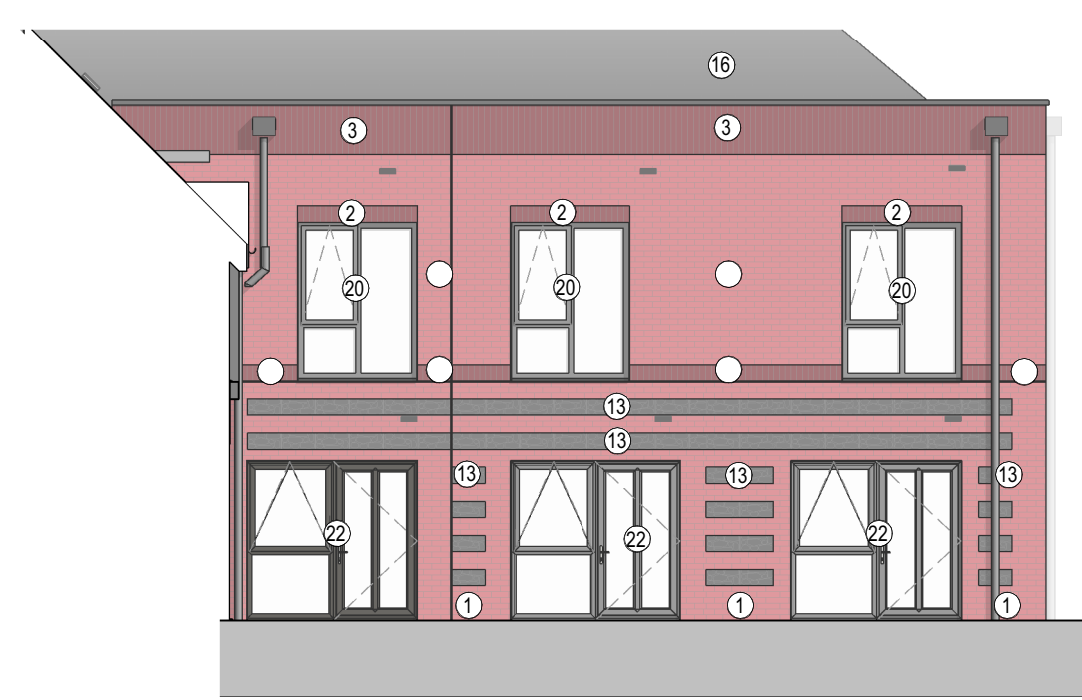
East Elevation (Hidden) planning 1:100
