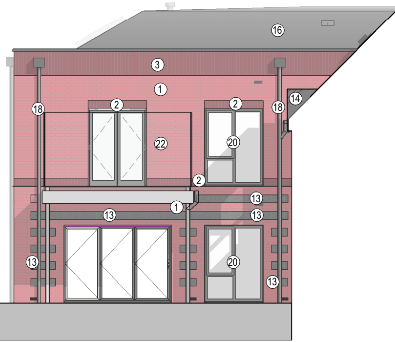
West Elevation (Hidden 2) planning 1:100
