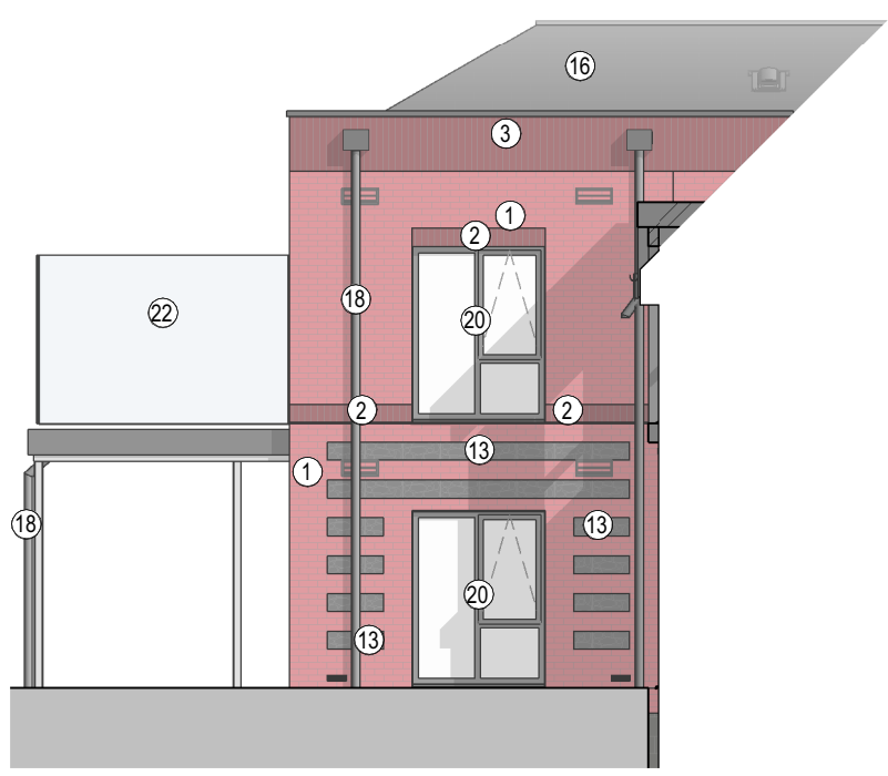
West Elevation (hidden) planning 1:100
