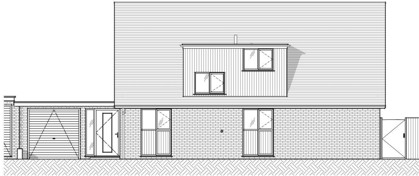
Existing Elevation - East
