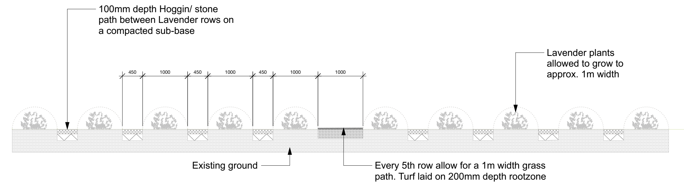
M02 Lavender field layout detail Scale: 1:50
