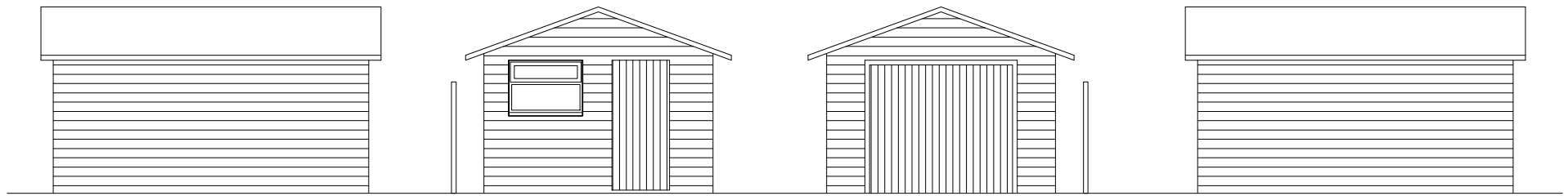
SIDE ELEVATION
