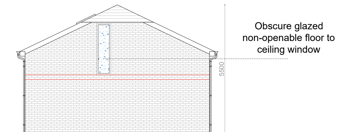
Proposed Left Elevation
