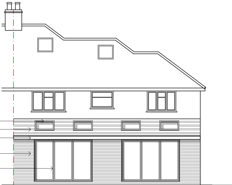
REAR ELEVATION (SOUTH FACING)
