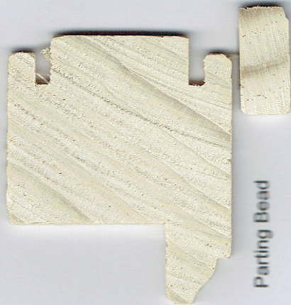
Sash side rail 50mm of which 20mm behind staff
