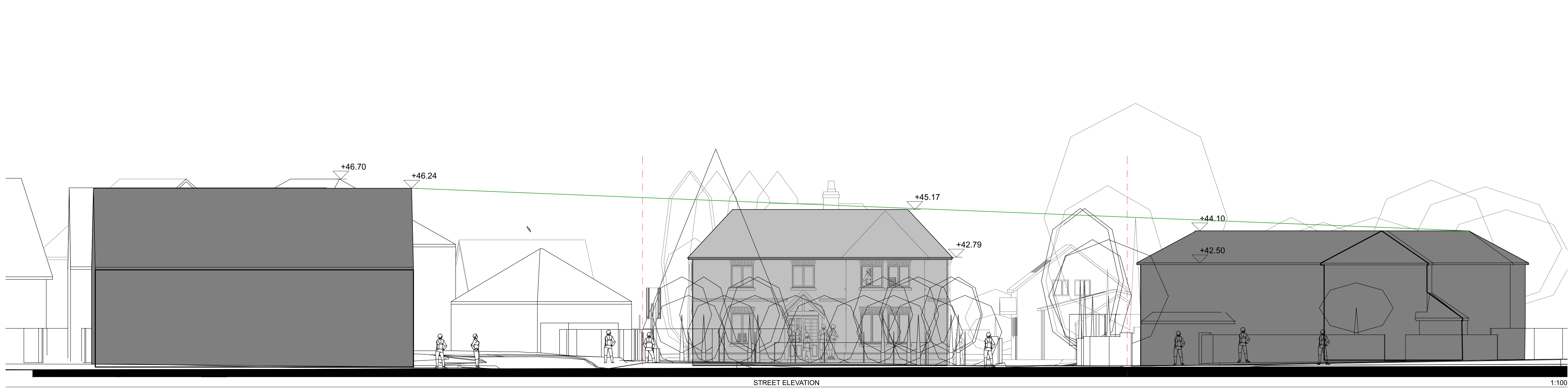
Height and pitch adjusted Building moved 0.8m east Simplified roof shape with hipped roofs/ valleys Added definition of elevation with hipped projection Set back 45m from road 47' roof pitch to match existing cottage Trees and Hedges shown
