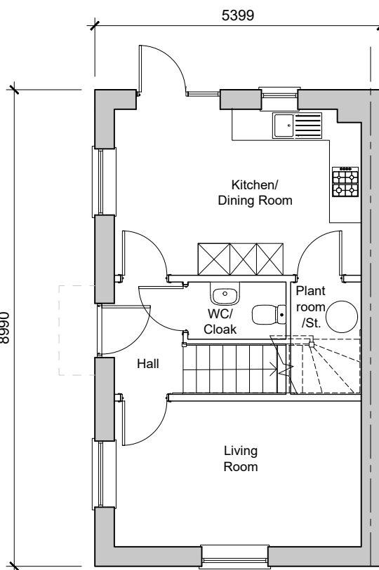
Ground Floor Plan 2-Bedroom House 76.83sqm / 827.04sqft GIA (by measured) Plots - 65, 82, 90, 97 Handed - 72, 73, 98
