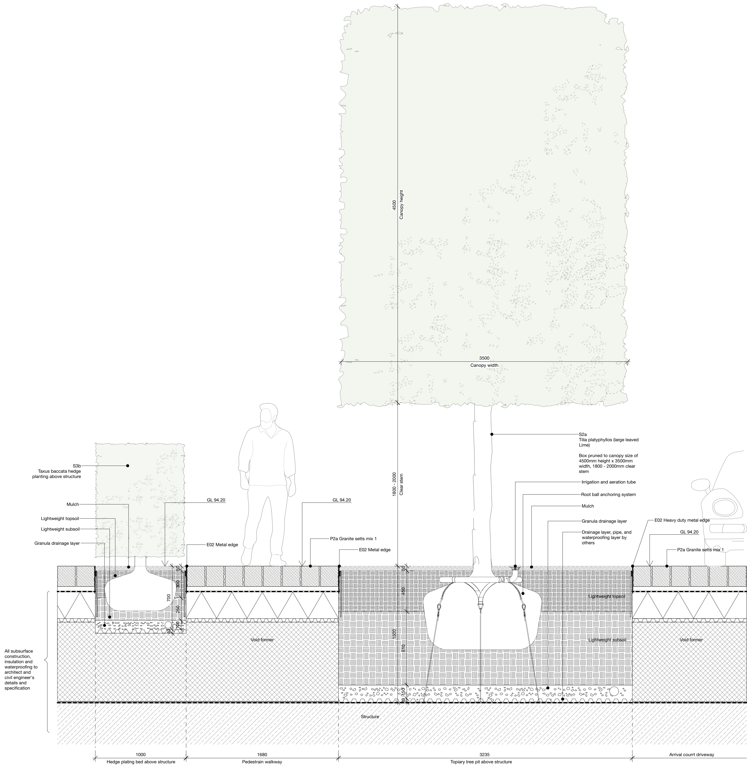
1 Soft landscape section - Arrival courtyard Scale: 1:20
