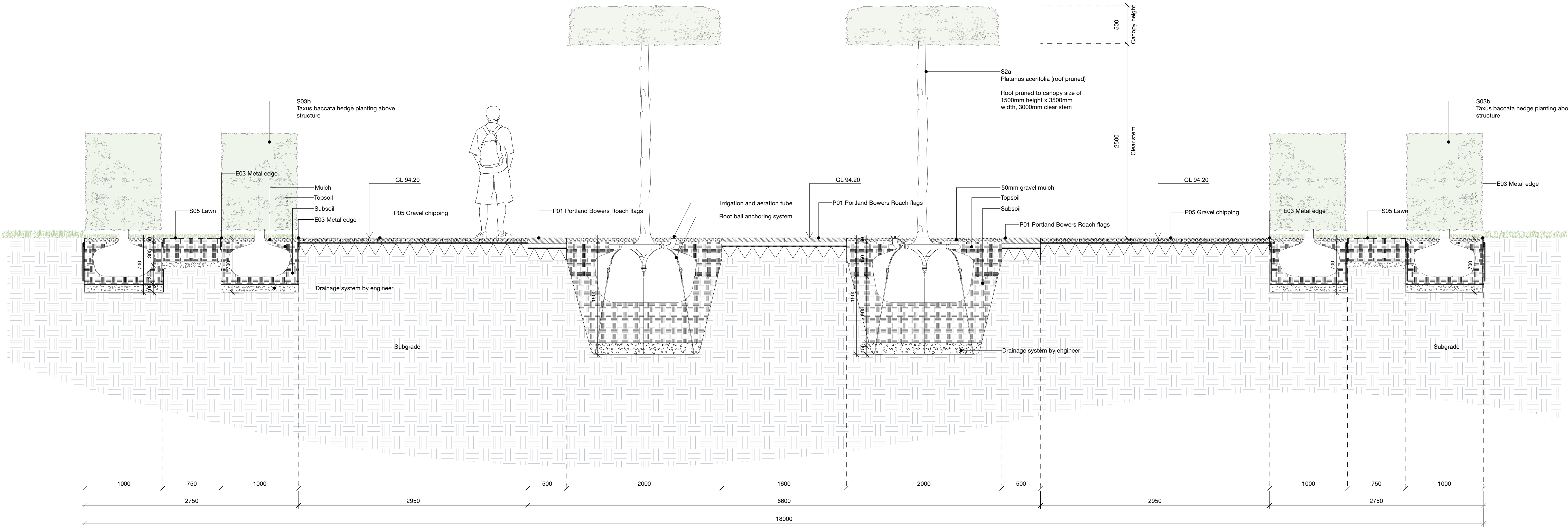
1 Soft landscape section - South garden Scale: 1:25
