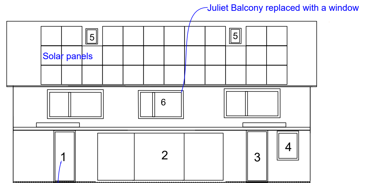
PROPOSED REAR ELEVATION WITH SOLAR PANELS AND VELUX WINDOWS 55X118
