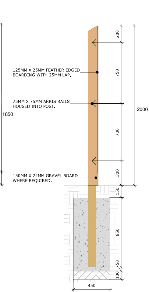
SECTION
