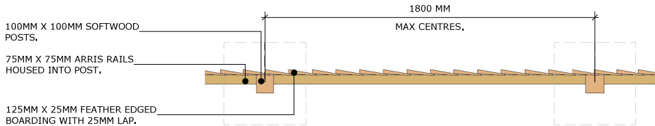
PLAN
