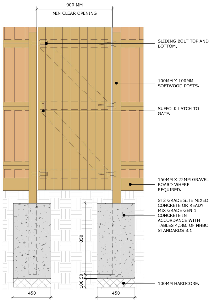
GATE ELEVATION
