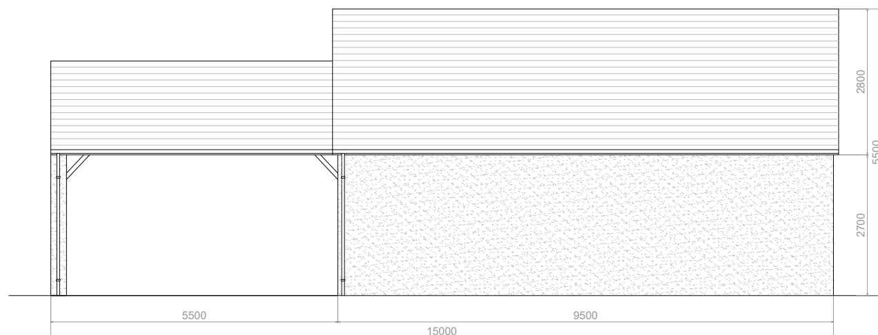
Rear Elevation
