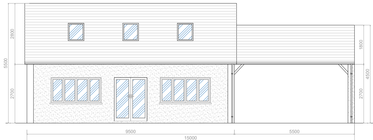
Front Elevation
