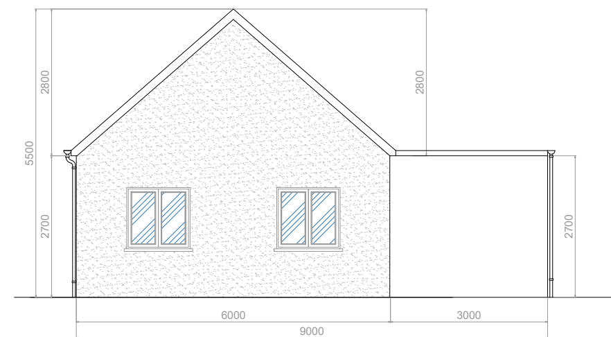
Left Elevation
