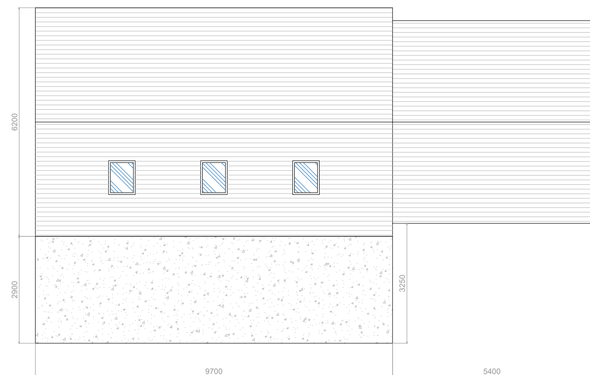
Roof Plan
