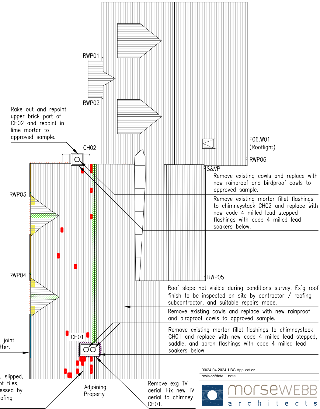
03 ROOF PLAN REPAIRS 1:100
