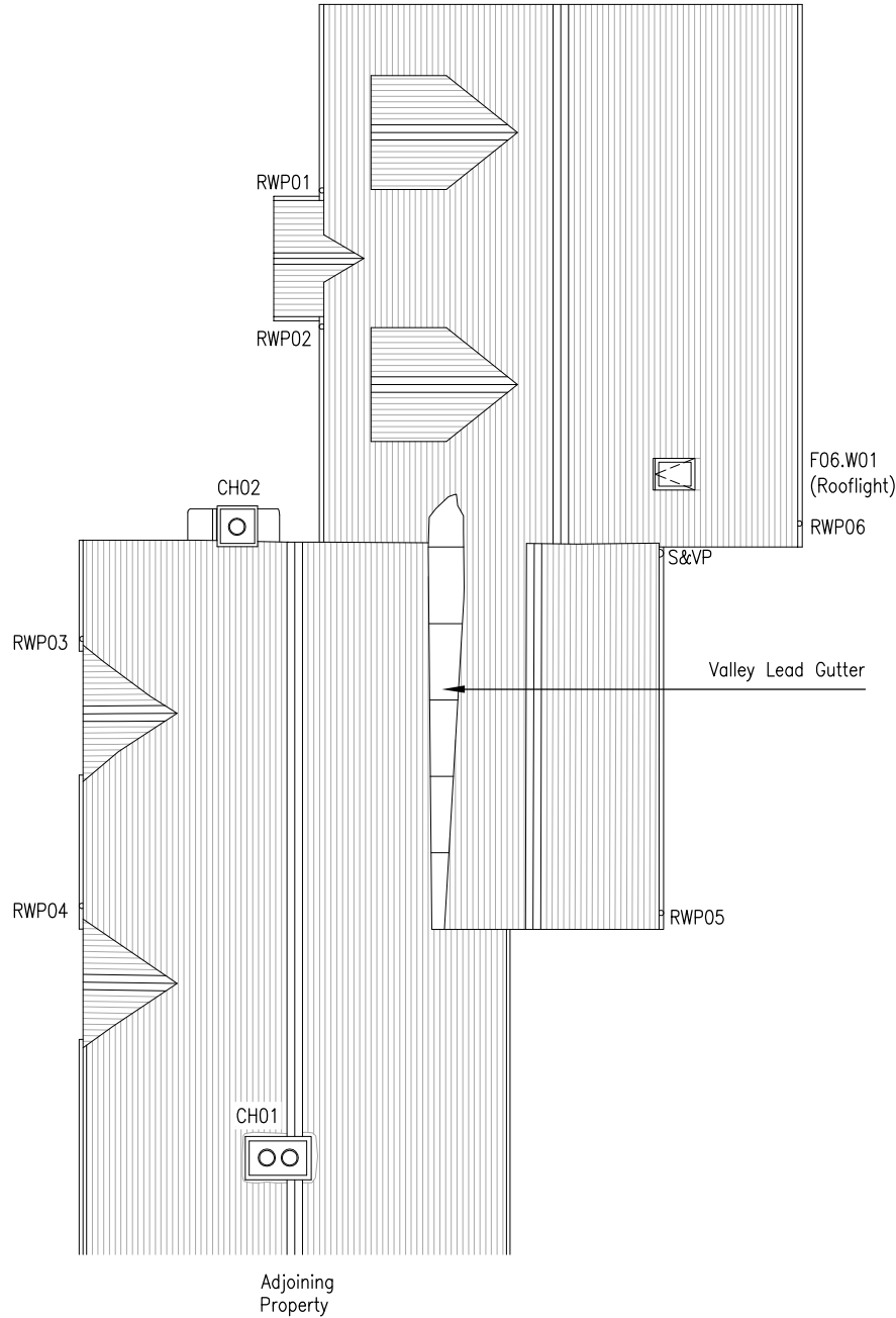
03 ROOF PLAN AS EXISTING 1:100
