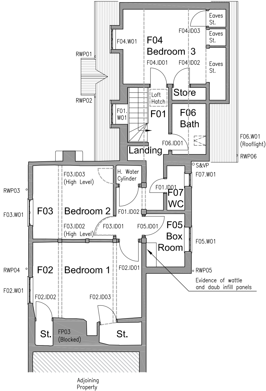
02 FIRST FLOOR PLAN AS EXISTING 1:100
