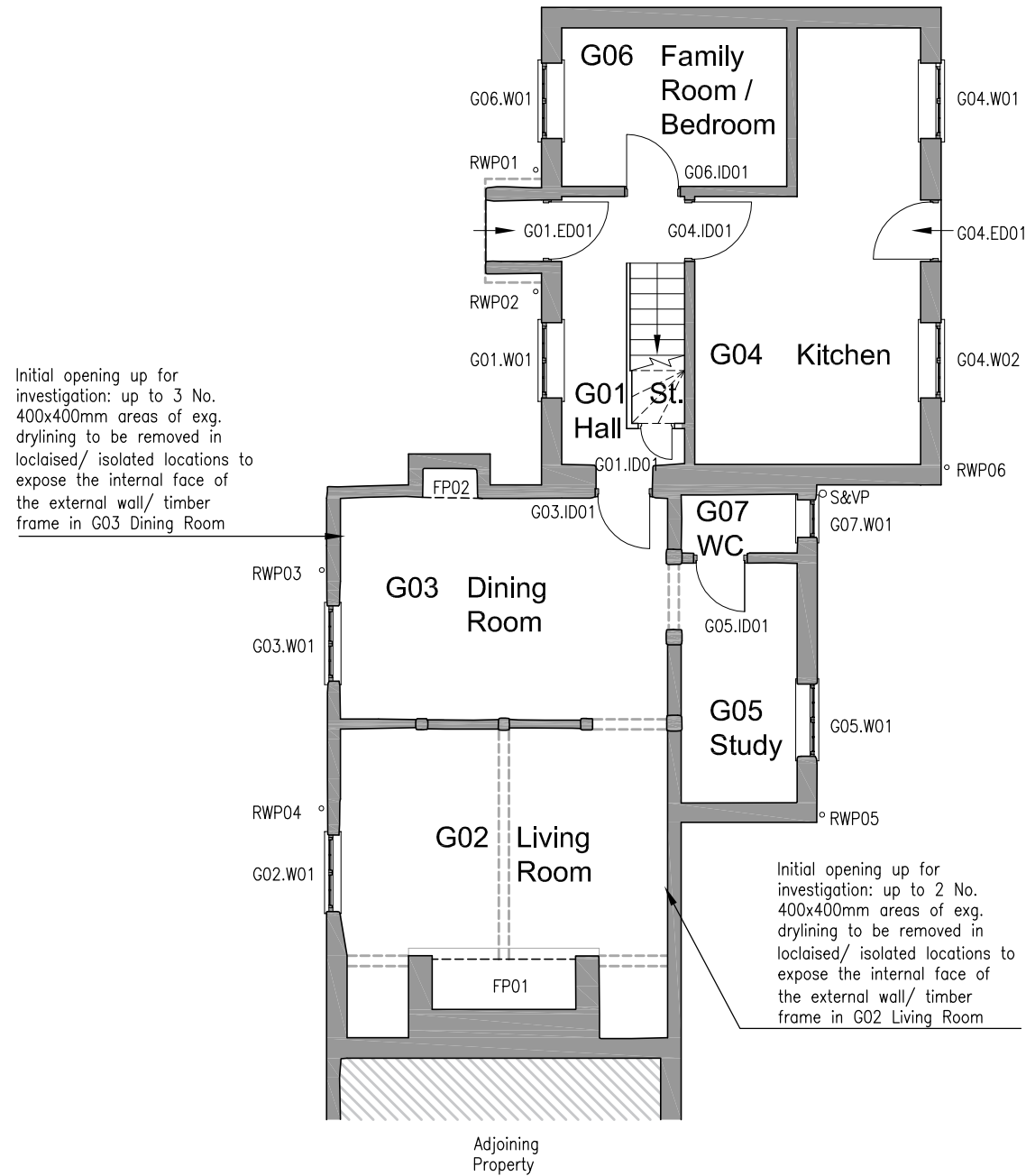
01 GROUND FLOOR PLAN AS EXISTING 1:100
