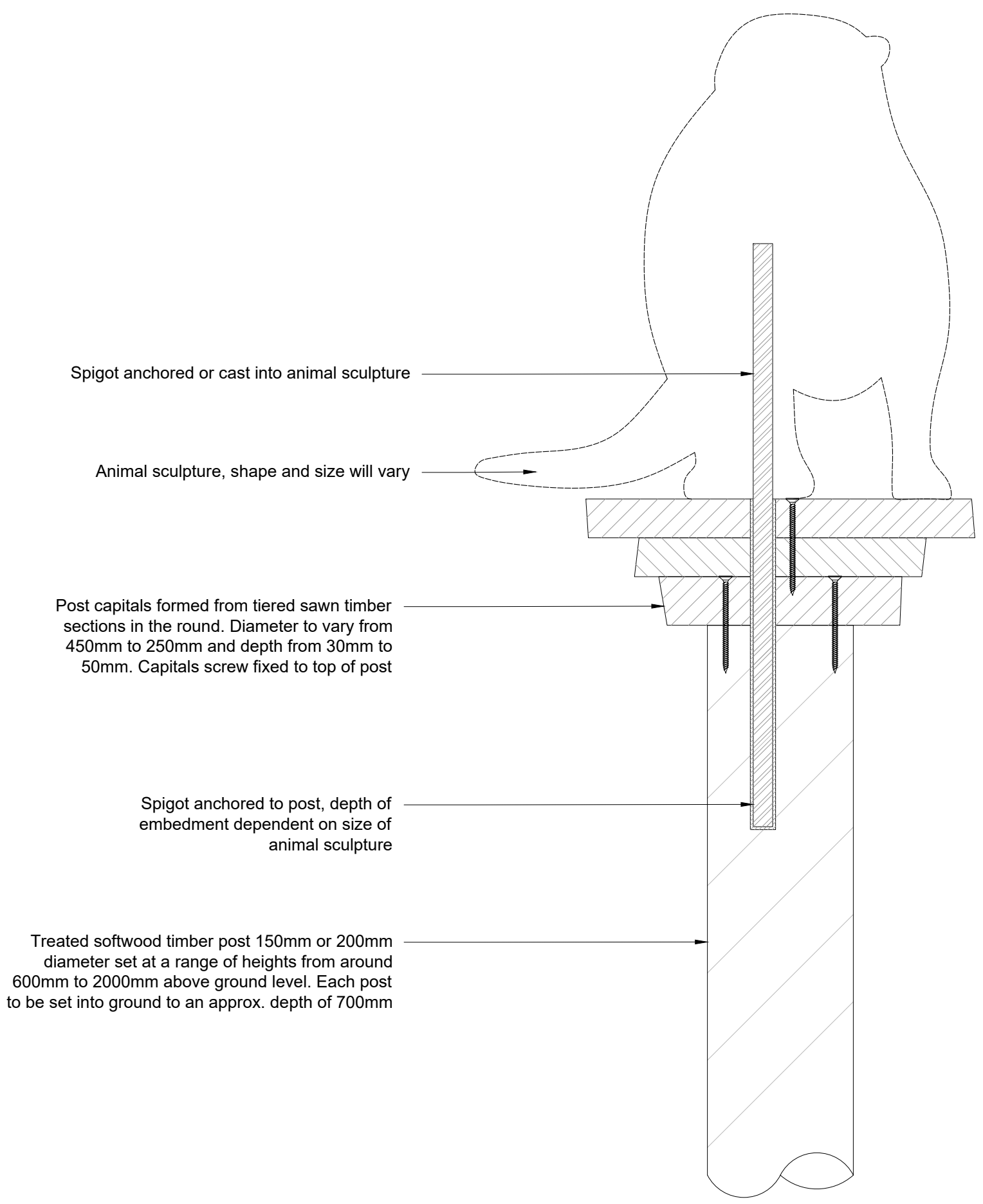
2 Animal sculpture and post attachment detail 1:5 @ A1
