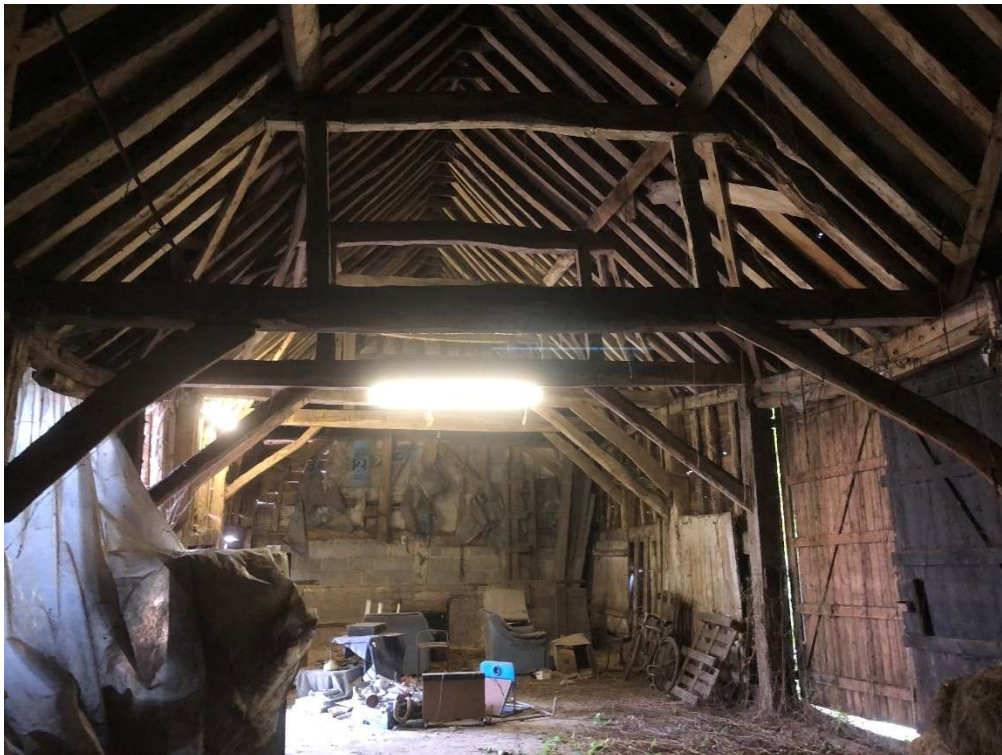
Photo 20 – Internal bays 2-6 facing East from Bay 1
