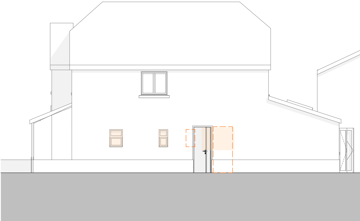
1:100 Proposed Right Side Elevation
