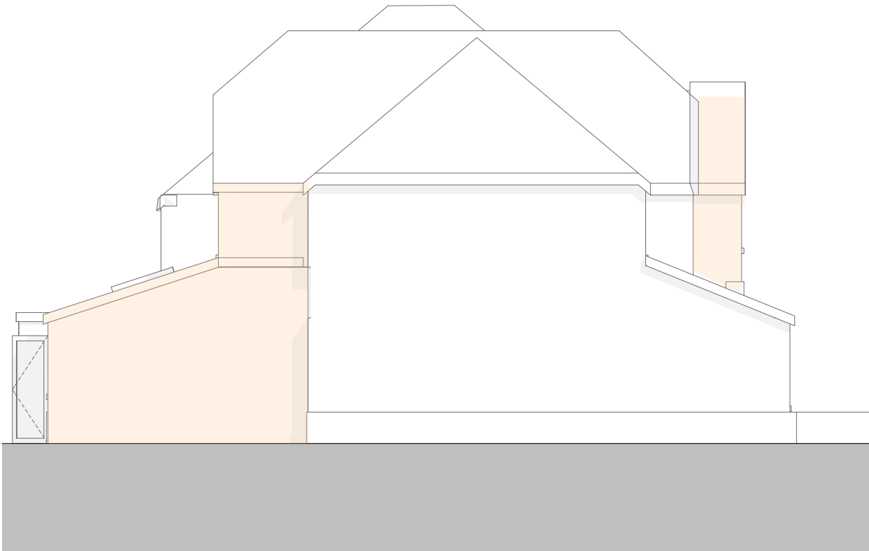
1:100 Proposed Left Side Elevation
