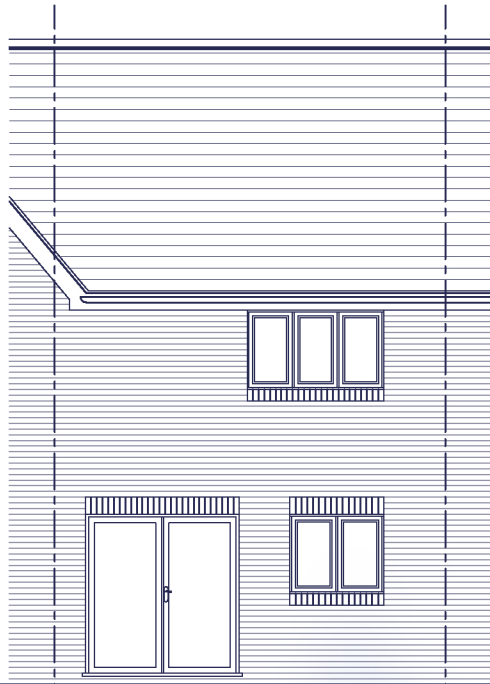
REAR ELEVATION
