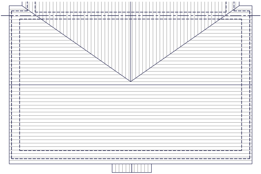
ROOF PLAN
