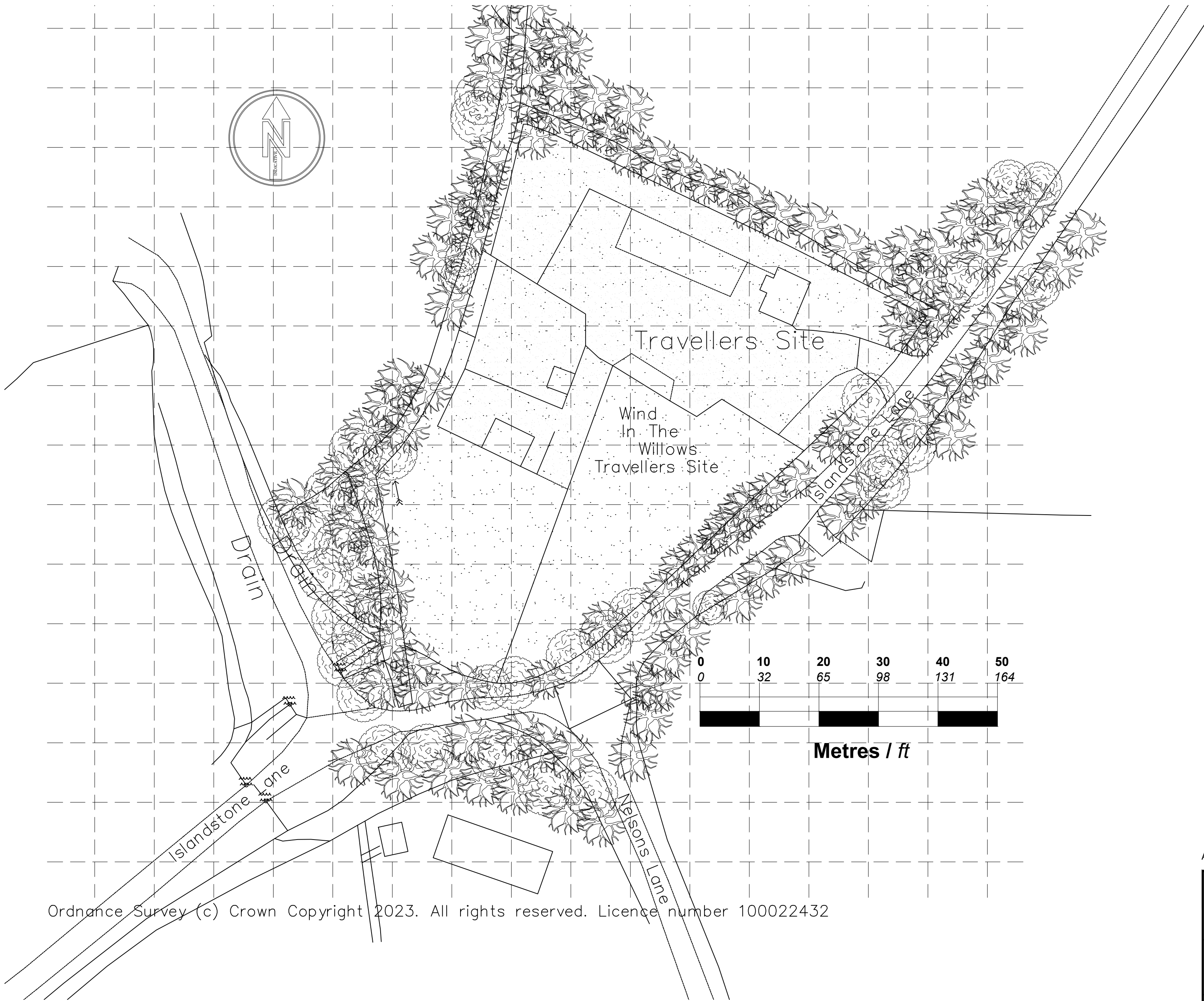
Site Layout Scale 1:500
